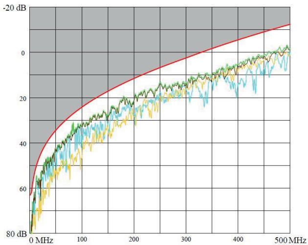
ACR (Attenuation to Crosstalk Ratio) (Ecart paradiaphonique)
