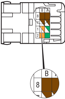
EIA 568A / EIA 568B
