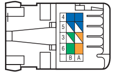
EIA 568B / EIA 568A
