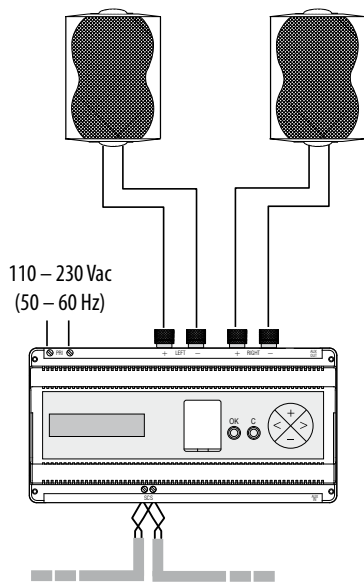
Wiring diagram with SCS BUS connected (the power amplifier plays back the sources from the 2-wire sound system).
