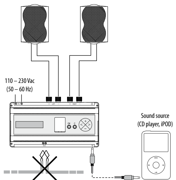
Wiring diagram with SCS BUS disconnected (the power amplifier is independent from the SCS BUS and plays back the source connected to the AUX IN input).
