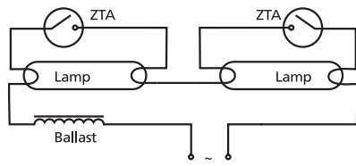
SERIES 220-240 V~
